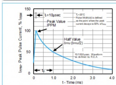
Figure 3 - Pulse Waveform
