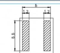
Recommended pad outline
